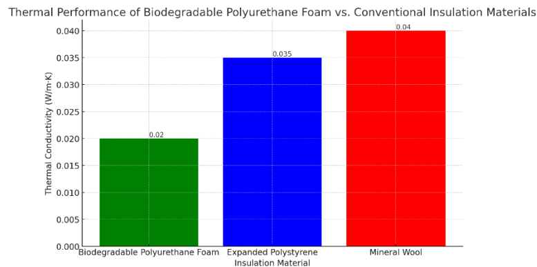
Fig. 1. Thermal performance of biodegradable Polyurethane foam vs conventional insulation material
