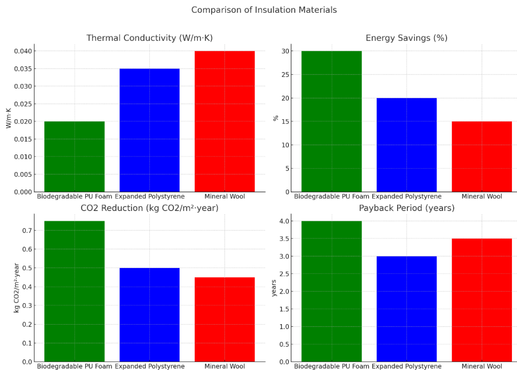
Fig. 2. Evaluation of the Efficiency of Biodegradable Foamed Polyurethanes
