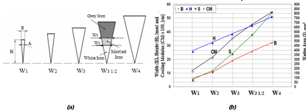
Fig. 1 Geometry of standard wedge shaped samples (a) and relationship of size parameters (b) [ W_c – clear chill; W_t – total chill] [ASTM A367]
