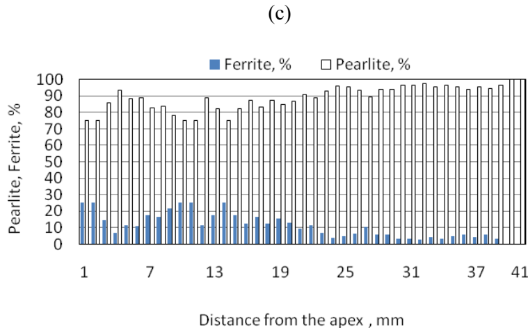
Fig. 4 Influence of inoculation and hold time after inoculation on metal matrix structure at different distances from the apex of W_{31/2} wedge sample, ASTM A 367 [a) inoculated iron; b) 5 min. hold; c) 10 min. hold; d) 11.5 min. hold and Re-inoculation] [Pearlite + Ferrite = 100 %]
