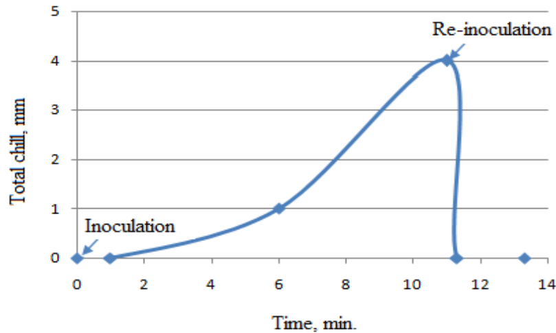
Fig. 2. Influence of inoculation and holding time on chill tendency [W 3 ½ wedge sample, ASTM A 367]
