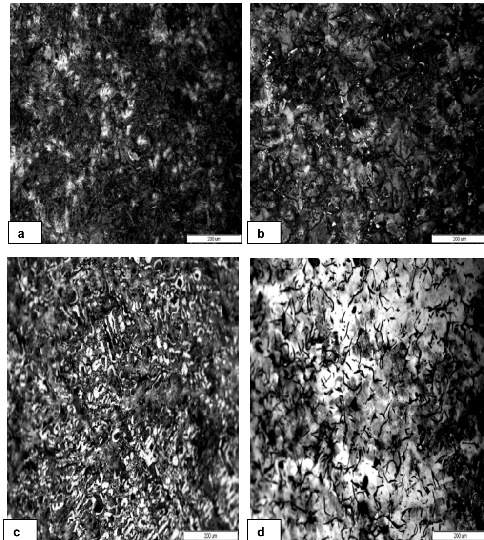
Fig. 3 Microstructure of cast irons at different hold time after inoculation [Nital 2 %]; [a) – inoculated iron; b) - 5 min. hold; c) - 10 min. hold; d) - 11.5 min. hold and re-inoculation] [23 mm from the apex, W_{3/2} wedge sample, ASTM A 367]
