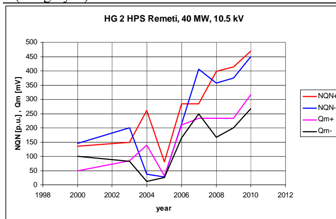
Fig. 9. NQN, Q_{\max} = f(\text{time})
