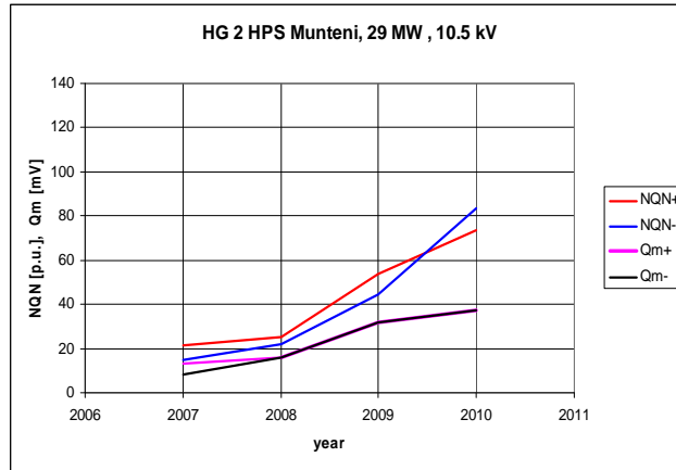
Fig. 11. NQN, Q_{max} = f(\text{time})
