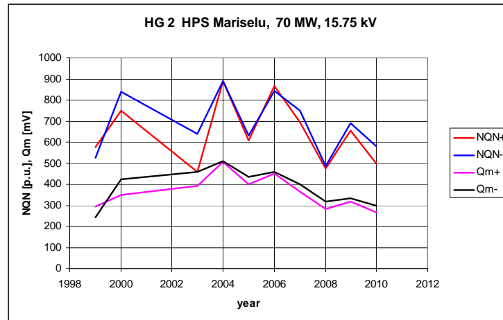
Fig. 4. \text{NQN}, Q_{\max} = f(\text{time})
