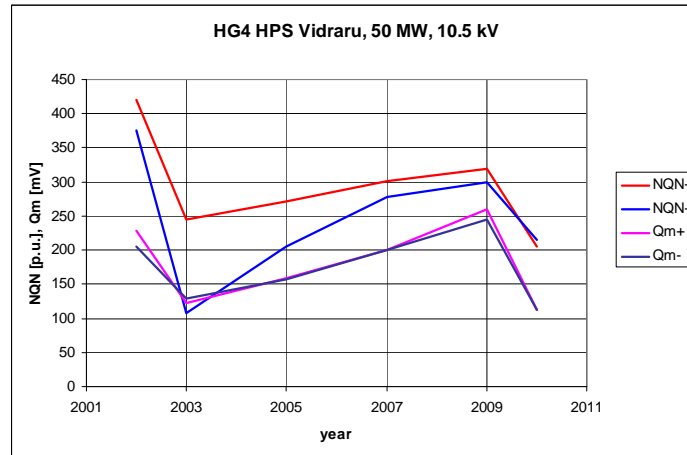
Fig. 6. NQN, Q_{\max} = f(\text{time})
