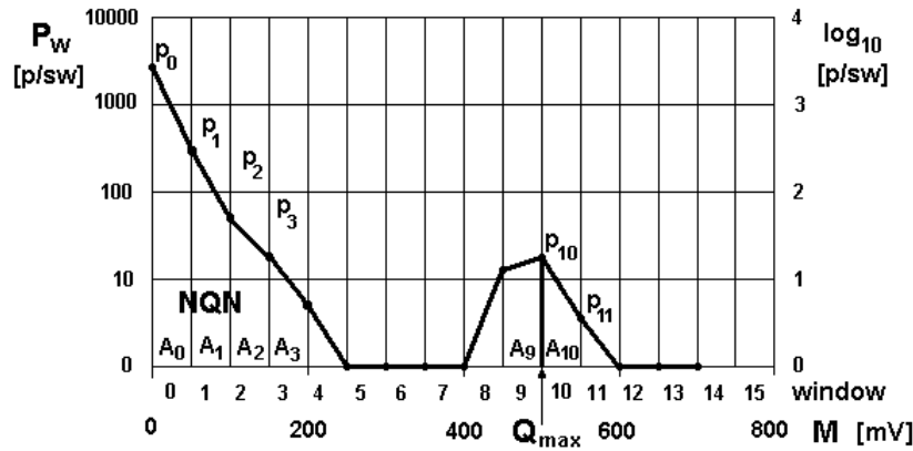
Fig. 3. Definition of the normalized quantity NQN and maximum magnitude Q_{\max}
