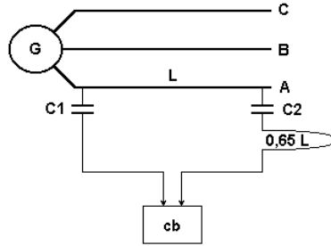
Fig.2. Coupler directional mounting system (BUS)
