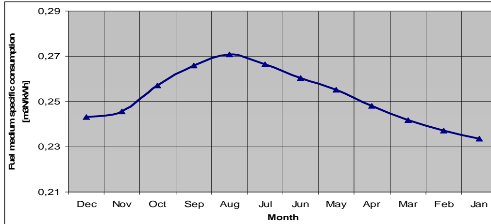
Fig. 5. Monthly variation of fuel medium specific consumption
