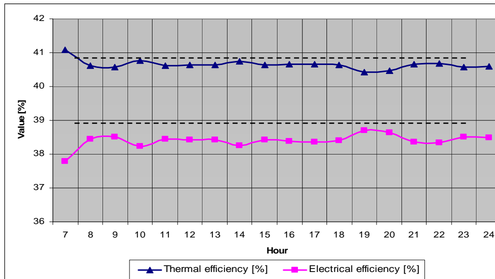
Fig. 3. Hourly variation of electrical and thermal efficiency for the cogeneration plant
