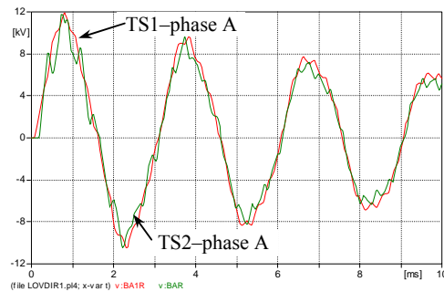
Fig.4. The line-to-ground voltages recorded at medium voltage terminals of the two transformers (TS1 and TS2).
