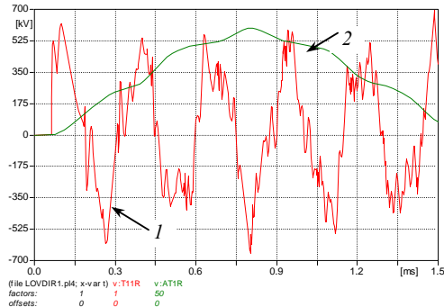
Fig.3. The line-to-ground voltages at primary (phase A – 1) and secondary (phase A' – 2; these values are multiplied by 50) terminals of 110/20 kV transformer due to the lightning stroke.
