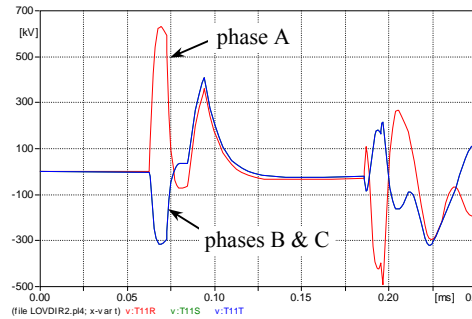
Fig. 6. The line-to-ground voltages at high voltage terminals of 110/20 kV transformer, after the propagation of the chopped lightning overvoltages along 110 kV line.
