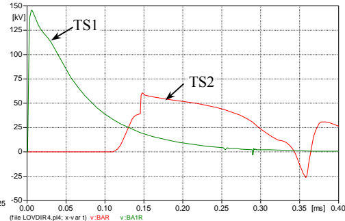
Fig. 7. The line-to-ground primary voltages at 20/0.4 kV terminals of transformers connected in TS1 and TS2 (for the last, the delay due to the propagation can be observed).
