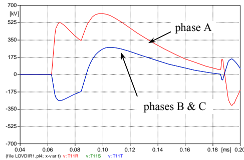
Fig.2. The line-to-ground voltages at high voltage terminals of 110/20 kV transformer, after the propagation of the surge along 110 kV line.
