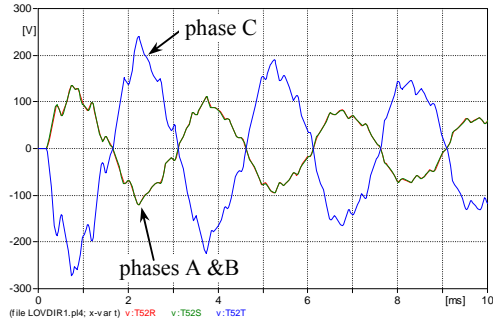
Fig.5. The line-to-ground voltages recorded at low voltage terminals of TS2 transformer.
