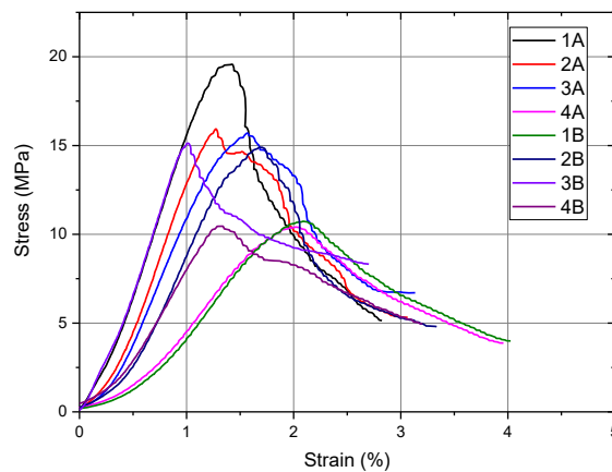
Fig. 10. Comparative compressive behaviour of all experimental samples
