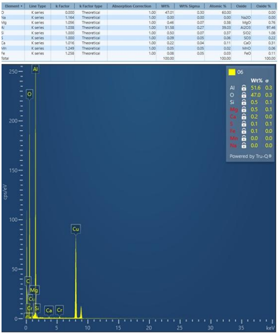
Fig. 3. EDS/EDX analysis of slag with particle size between 1 and 2 mm
