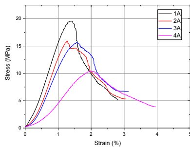
Fig. 8. Compressive behaviour of experimental samples R1(1A)-R4(4A)
