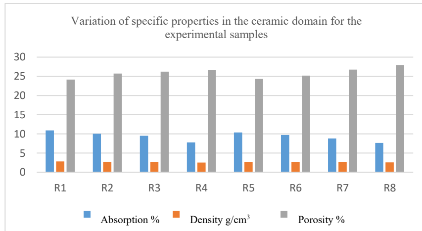
Fig. 7. Variation of specific quality characteristics of ceramic and refractory materials for the eight experimental samples
