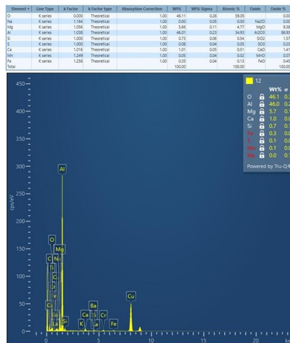
Fig. 1. EDS/EDX analysis of slag with particle size below 0.5 mm
