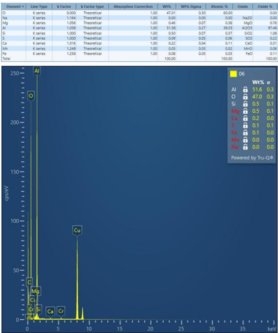
Fig. 2. EDS/EDX analysis of slag with particle size between 0.5 and 1 mm
