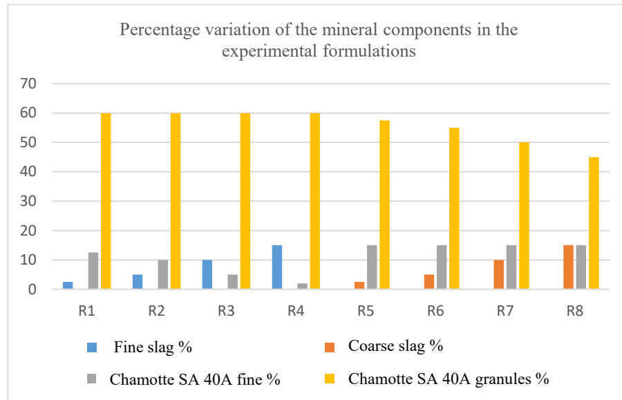
Fig. 5. Proportion of components in the experimental manufacturing formulations
