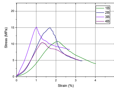
Fig. 9. Compressive behaviour of experimental samples R5(1B)-R8(4B)
