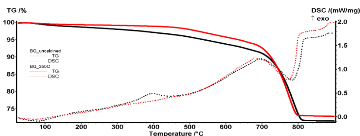
Fig. 1. TG/DSC curves of the Fe 3 O 4 -doped bioactive glass samples in the RT–900 °C range.
