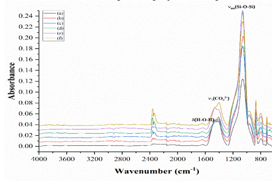
Fig. 7. FTIR-ATR spectra of bioglass samples: before (a) and after immersion in SBF for 1 day (b), 3 days (c), 7 days (d), 14 days (e) and 28 days (f), in 4000-600 \text{cm}^{-1} wavenumber range
